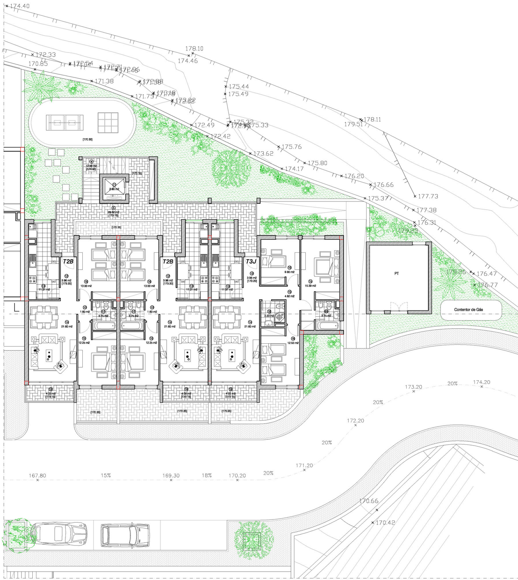
PLANTA COTA 173.20 (BLOCO B)
